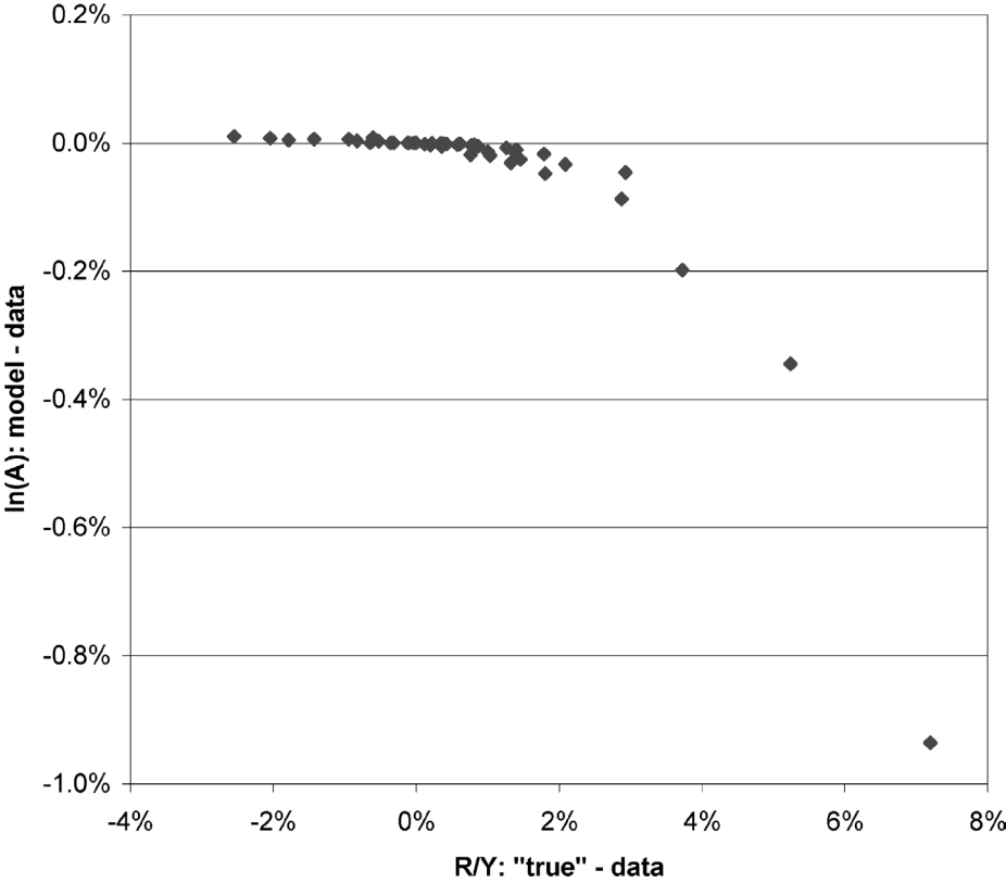
Figure 4. Deviations of the model from the data for research intensity and productivity.
