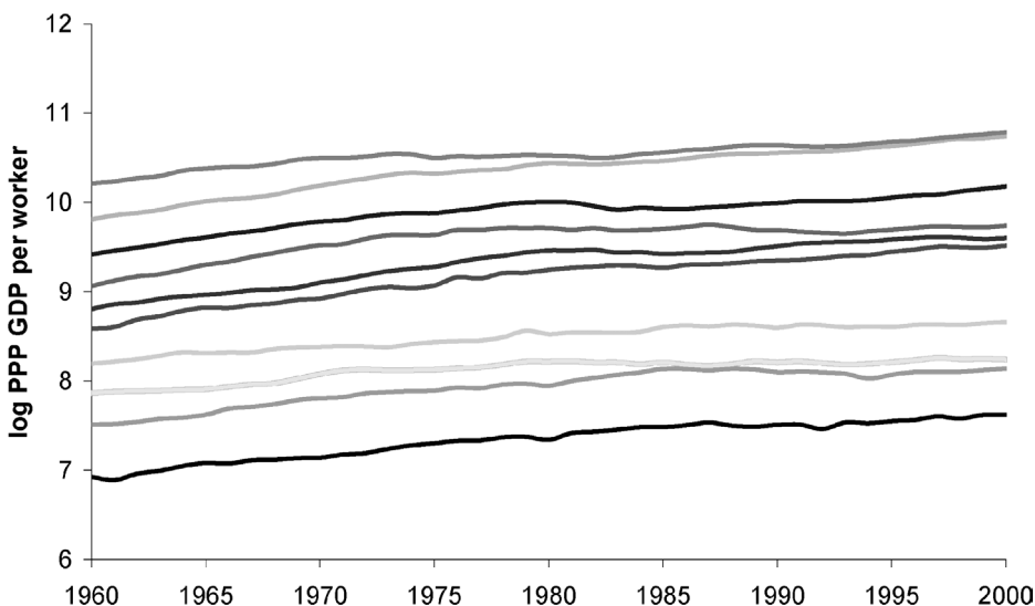
Figure 3. The evolution of income for 1960 deciles. Source: Penn World Table 6.1.
