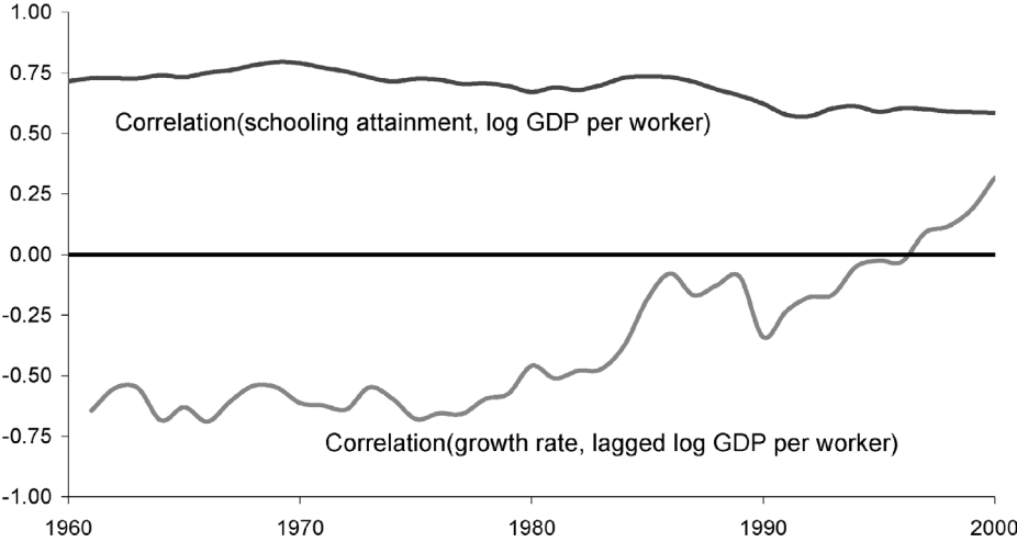
Figure 2. OECD incomes correlate negatively with growth rates, positively with investment schooling. Source: Penn World Table 6.1 and Barro and Lee (2000) data for 21 OECD Countries.
