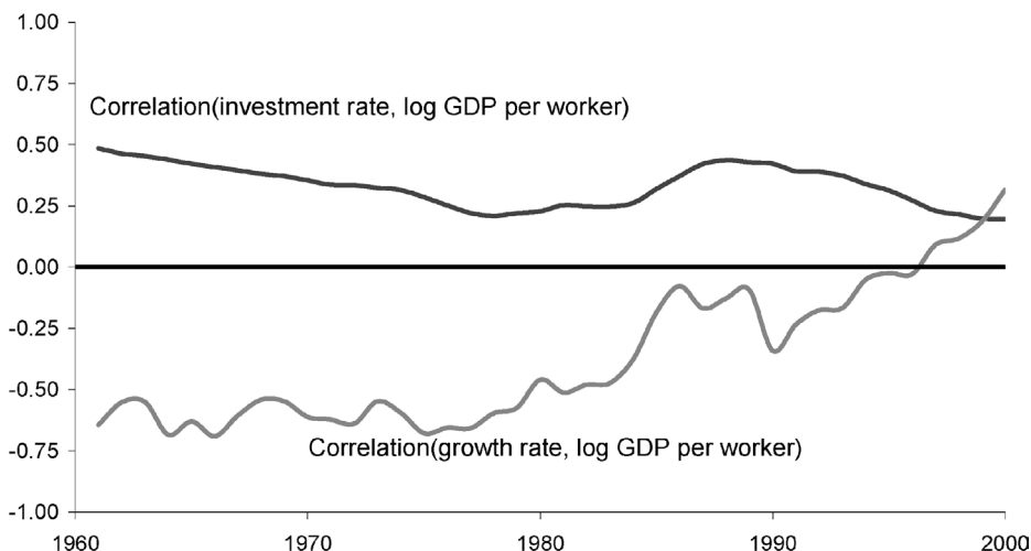
Figure 1. OECD incomes correlate negatively with growth rates, positively with investment rates. Source: Penn World Table 6.1 data on 23 OECD Countries.
